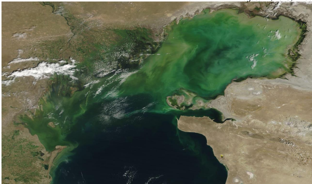
Fig.1 Space image of the Caspian Sea, August 19, 2025 (NASA/GSFC)
