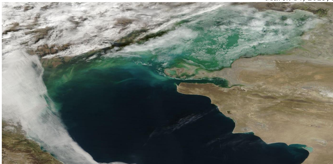
Fig.1 Space image of the Caspian Sea, March 14, 2025 (NASA/GSFC)
