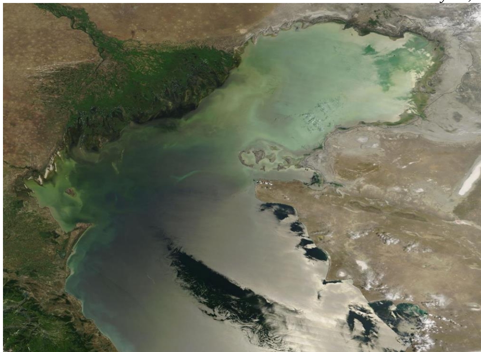
Fig.1 Space image of the Caspian Sea, July 23, 2026 (NASA/GSFC)
